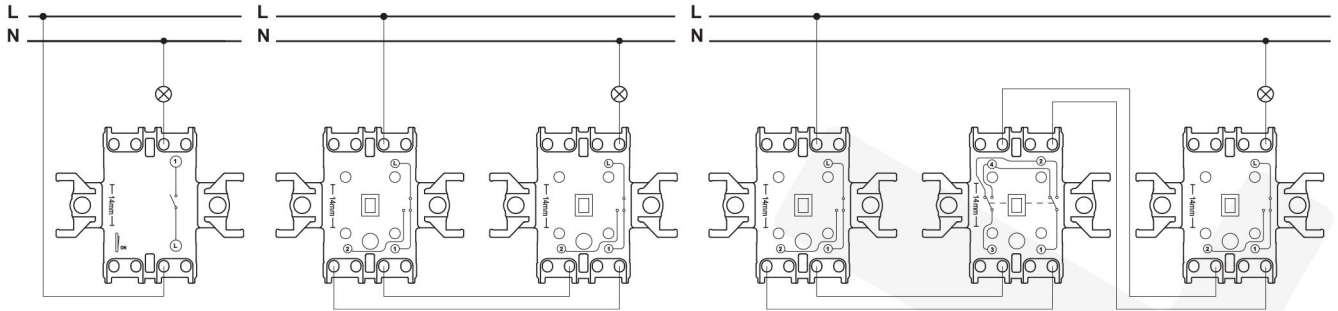
1-way switch
